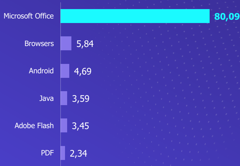
Distribution of exploits used in attacks by type of application attacked (in %)
