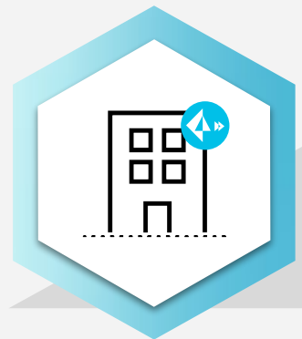
SD-WAN
